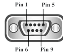
RS232 Pinout (9 Pin Male)
